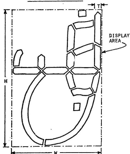
Fig. 6. The proposed line-segment display for Farsi alphanumeric information.
