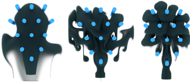
Fig. 6. Larger bases resolve thinner obstacles, as shown in the CYLINDERS scene. The basis rank from left to right is r = 200 , r = 1000 , and r = 7000 .
