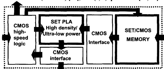
Figure 19. Hybrid SET/CMOS ULSI architecture, after [26].
