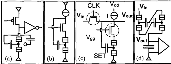
Figure 18. Hybrid SET/CMOS ICs: (a) NVM circuit for programmable logic (undulated-film SET) [26], (b) multiple-valued SRAM cell (PADOX) [32], and (c, d) quantizers [34, 35].
