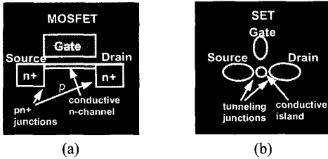
Figure 5. Schematic of: (a) MOSFET and (b) C-SET.
