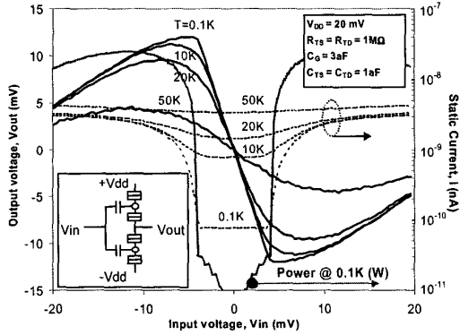
Figure 13. C-SET inverter static characteristic, V_{out} vs. V_{in} .
