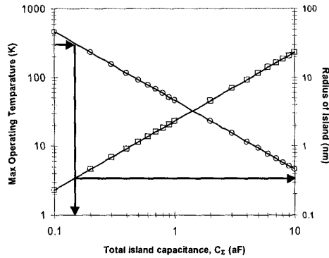
Figure 10. Maximum C-SET operating temperature, T_{max} , (with Kiriwara's criteria [19]) vs. total island capacitance, C_\Sigma .
