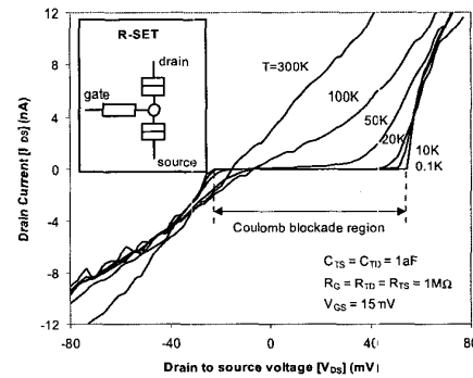
Figure 9. R-SET I_{DS} - V_{DS} simulated [18] characteristics for various temperatures, T , highlighting Coulomb blockade.
