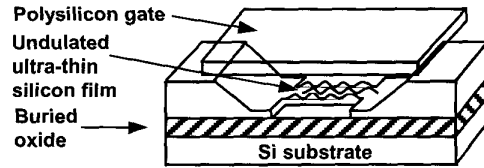
Figure 11. SOI-SET with undulated ultra-thin SOI film [26].
