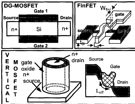
Figure 3. Emerging MOSFET device architectures.
