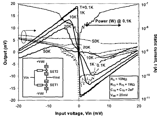
Figure 14. R-SET inverter static characteristic, V_{out} vs. V_{in} .
