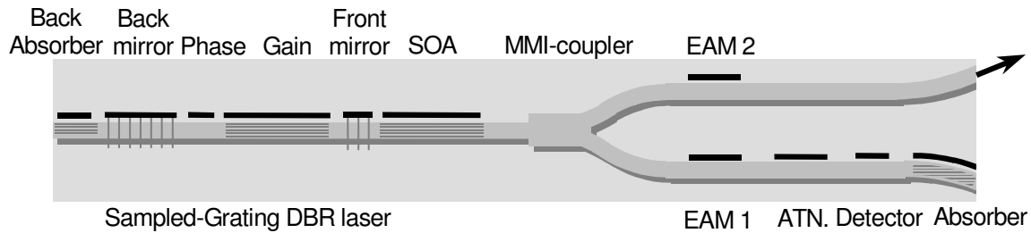
Fig. 8. Schematic of integrated photonic circuit.
