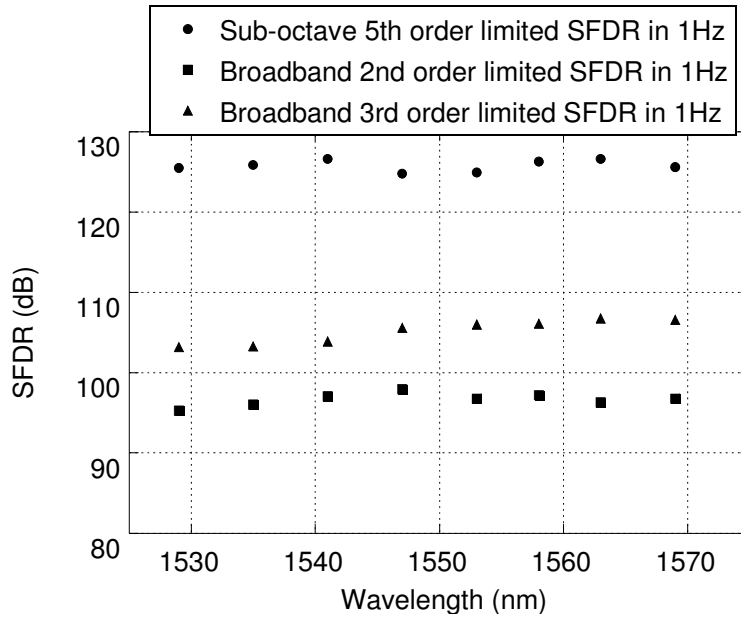
Fig. 1: Summary of measured EA SFDR when biased for broadband linear operation and biased for sub-octave linear operation, normalized to 1 Hz noise bandwidth.
