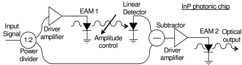
Fig. 7. Operational schematic of broadband linearization scheme.
