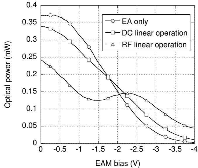
Fig. 14. Measured modulator extinction using the EAM only, and for the bias points of DC and RF linearized operation, respectively
