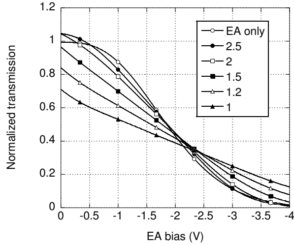
Fig. 13. Simulated linearized DC extinction curves for different ratios of equivalent EAM V_{\pi} to Mach-Zehnder V_{\pi}
