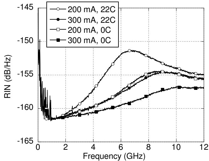
Fig. 5. Measured RIN at 200mA and 300 mA and at 20 deg C and 0 deg C.
