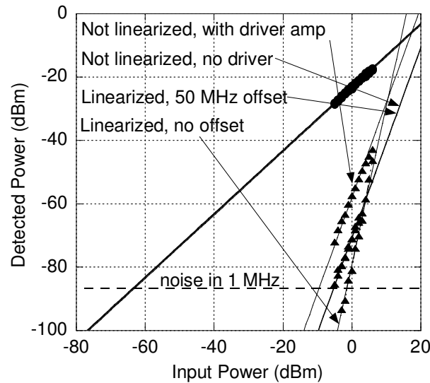
Fig.10: SFDR of the predistorted transmitter with and without 50 MHz frequency offset from setting, and not predistorted with and without driver. The input power has been adjusted to facilitate comparison.
