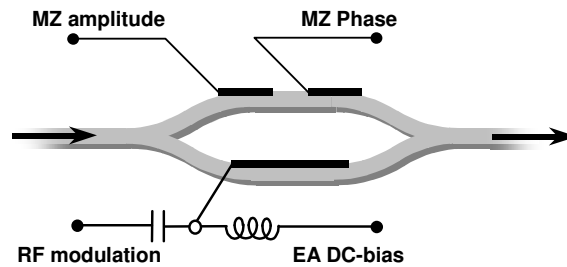
Fig. 12. Simple schematic of proposed modulator.
