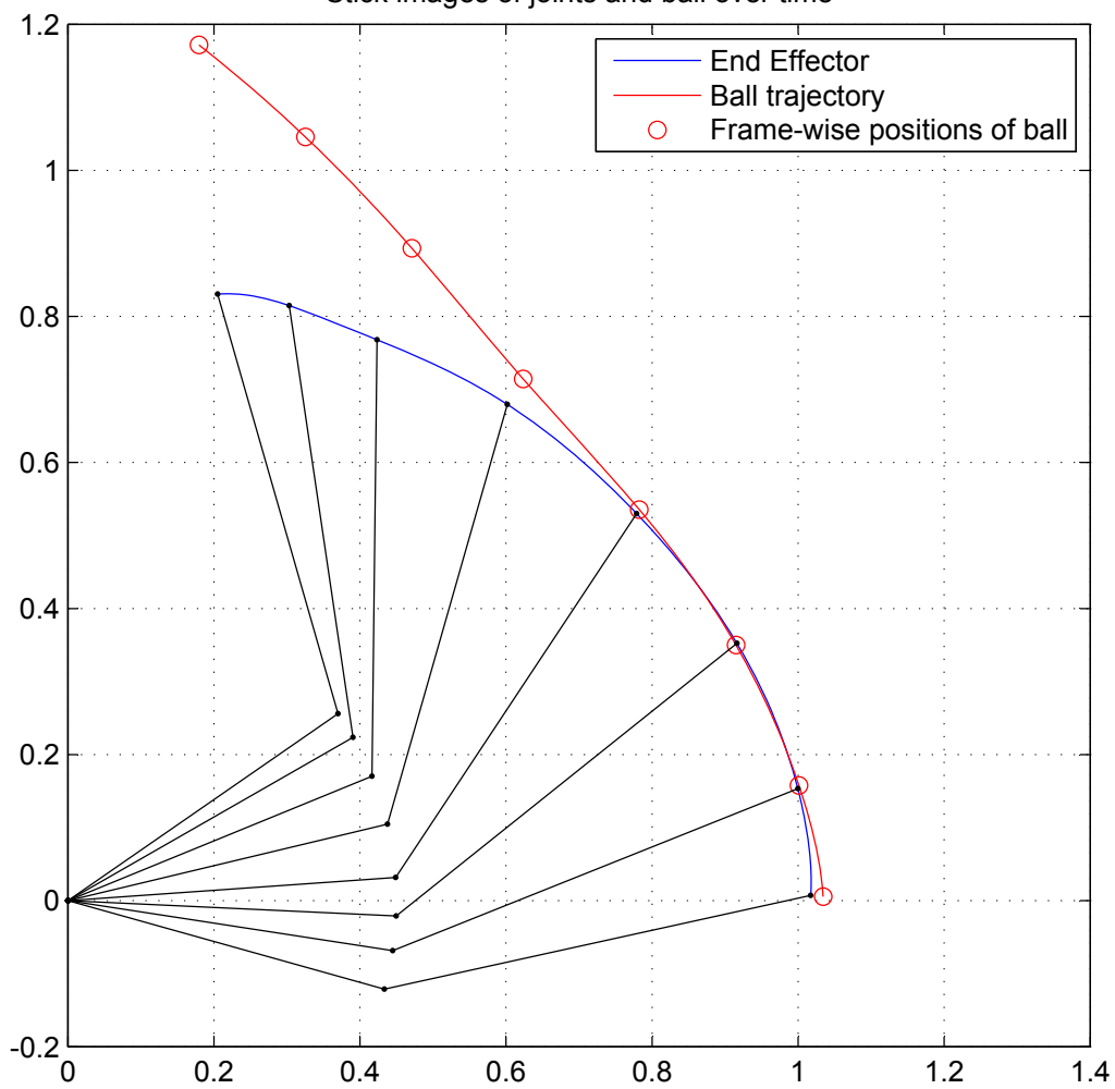
Stick images of joints and ball over time
