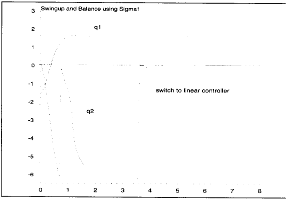
Fig. 5. Swing up motion of the Acrobot using \Sigma_1 .
