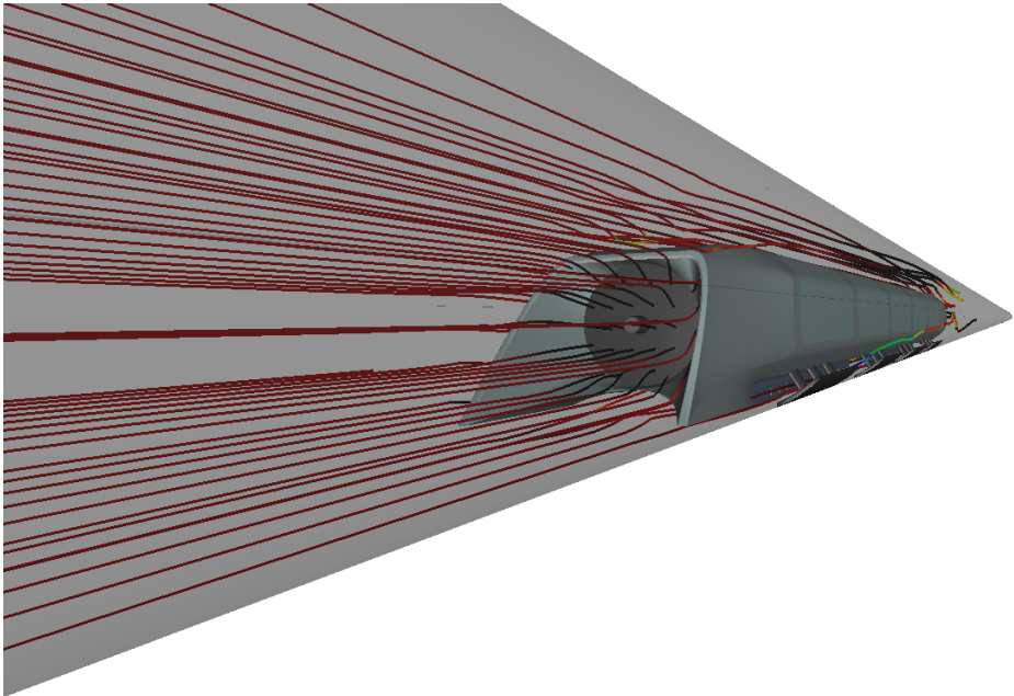
Figure 7. Streamlines for capsule traveling at high subsonic velocities inside Hyperloop.
