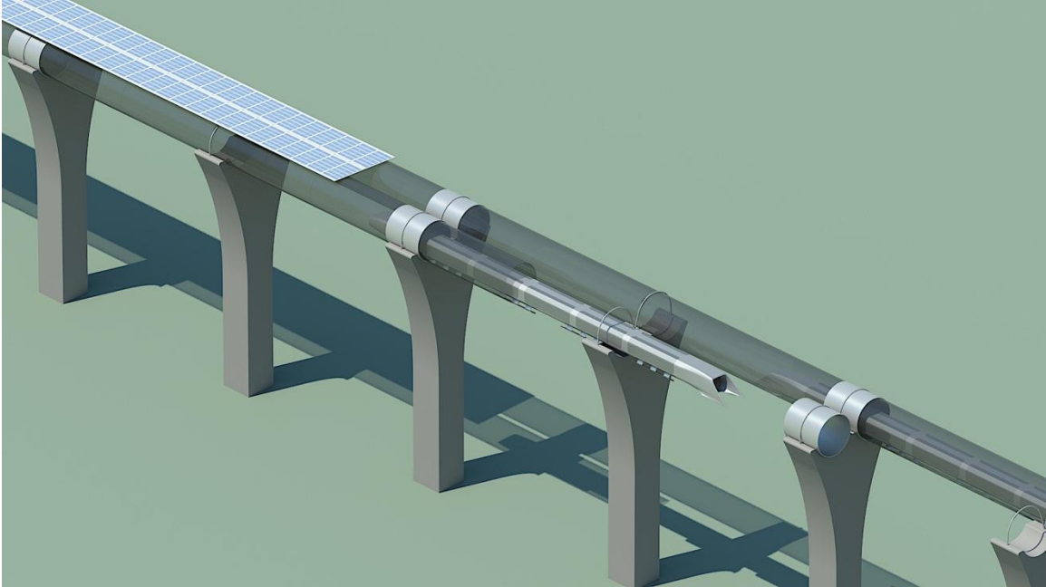
Figure 14. Hyperloop capsule in tube cutaway with attached solar arrays.
