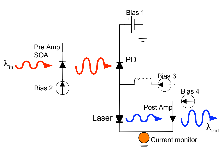
Direct Drive Configuration
