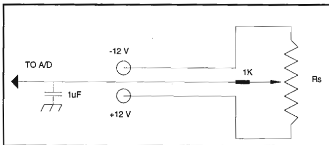
WI- 10 Wiring the seesaw angle sensor
