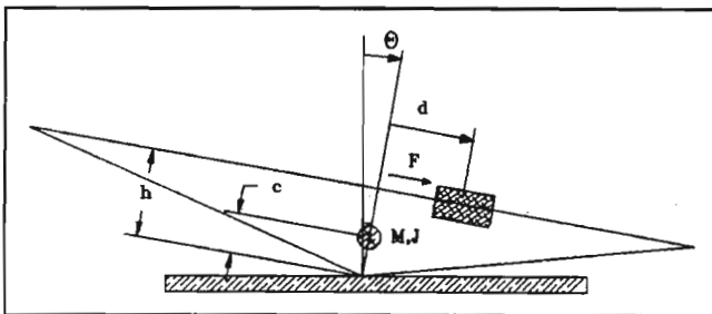
SS 2 Simplified model for seesaw experiment
