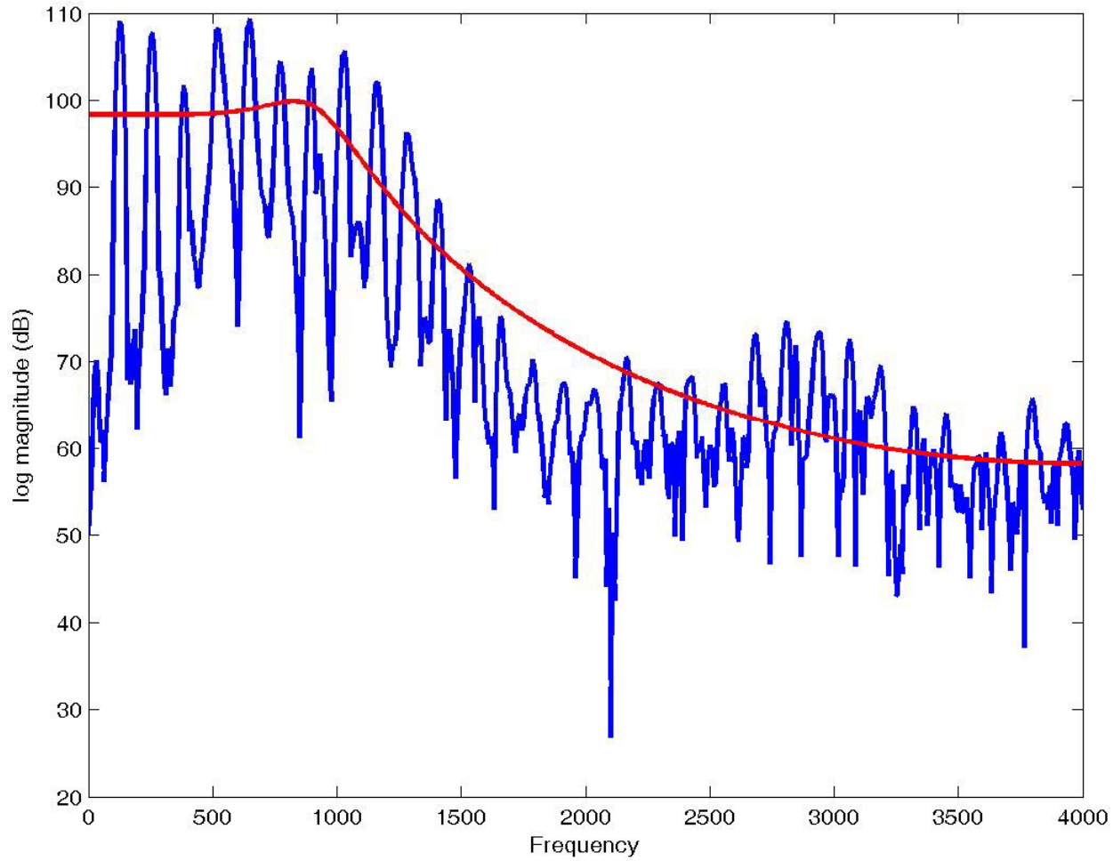
Frequency Response of Speech for LPC order p = 4
