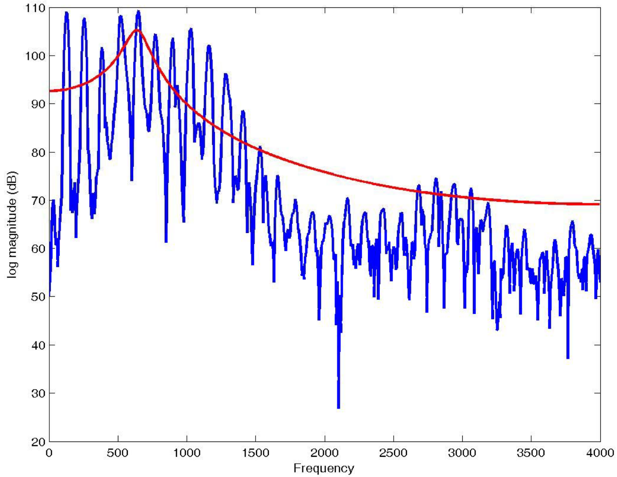
Frequency Response of Speech for LPC order p = 2
