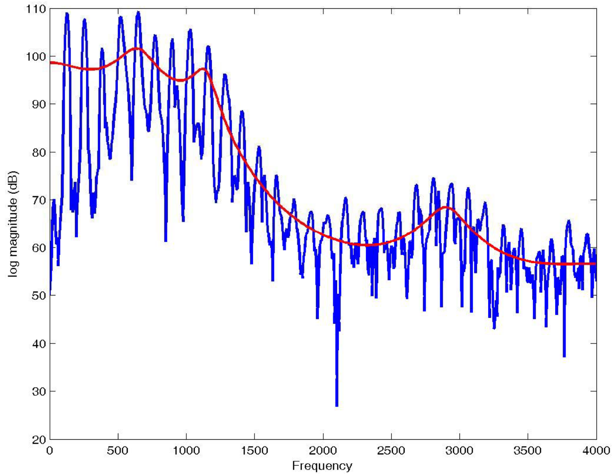
Frequency Response of Speech for LPC order p = 10
