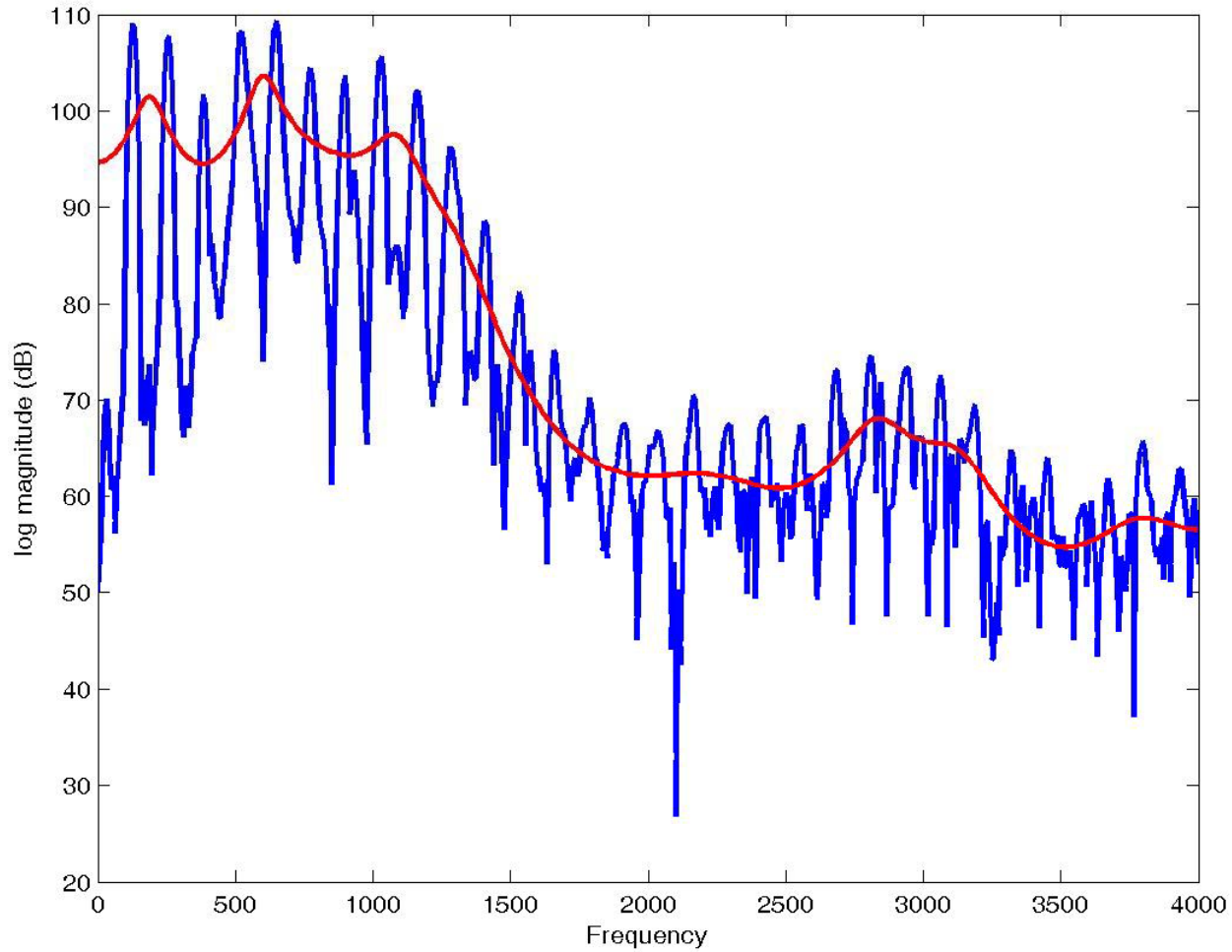
Frequency Response of Speech for LPC order p = 20
