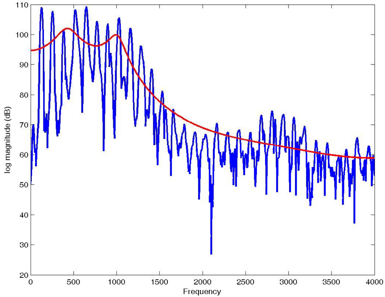
Frequency Response of Speech for LPC order p = 6
