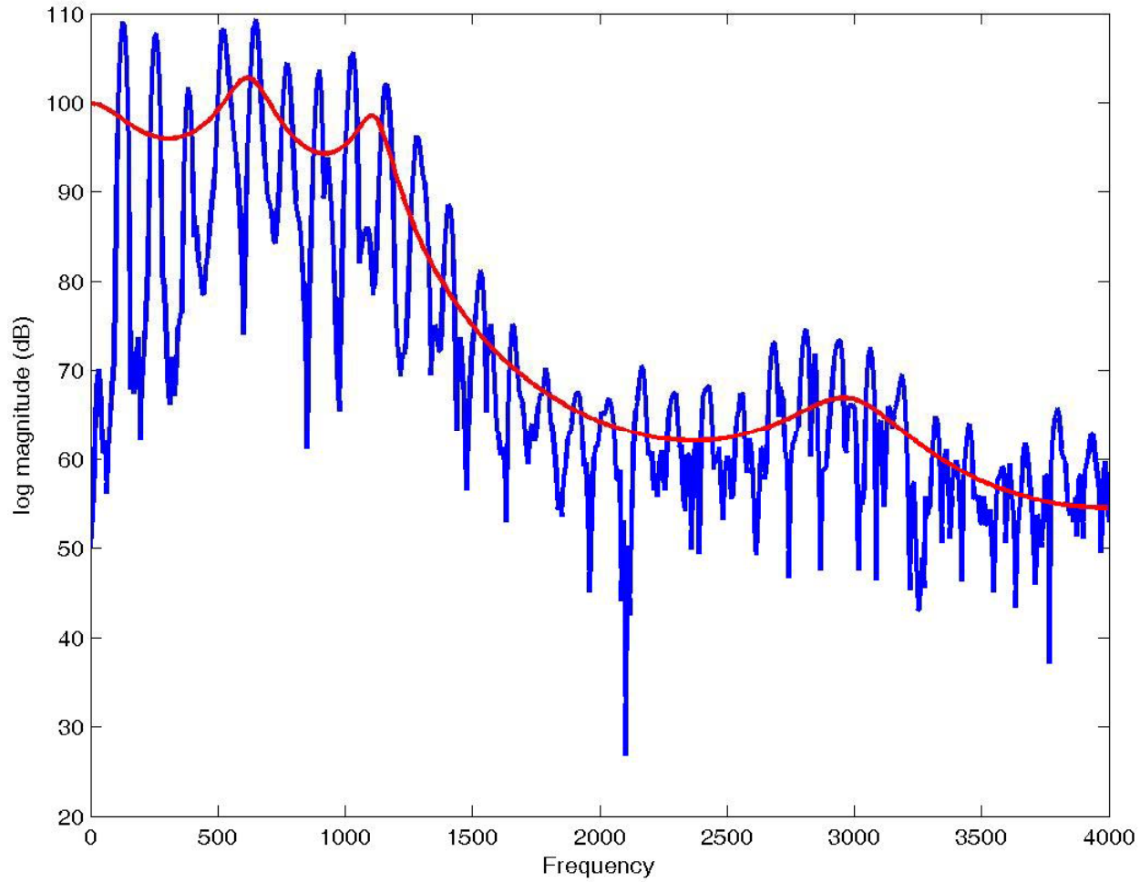
Frequency Response of Speech for LPC order p = 8
