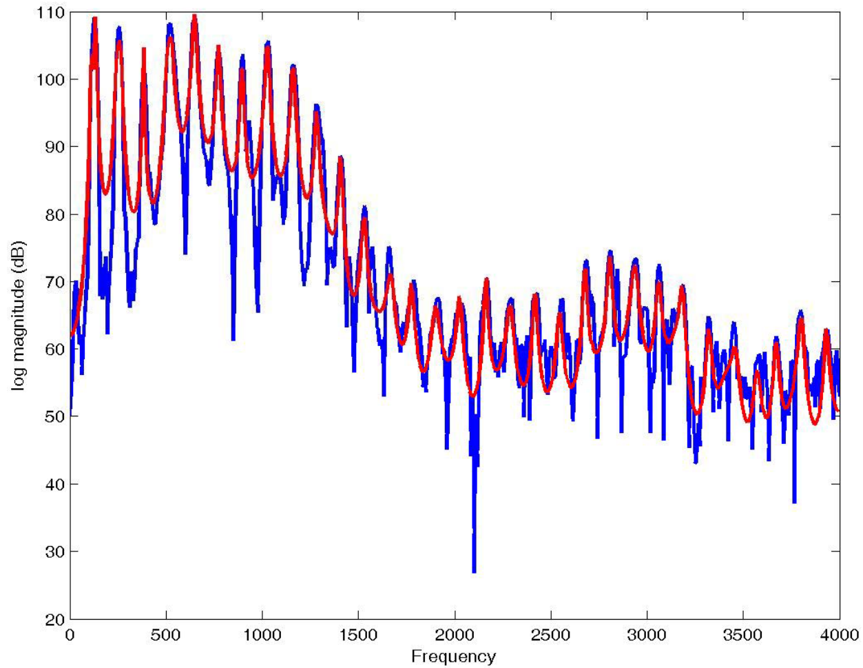
Frequency Response of Speech for LPC order p = 100
