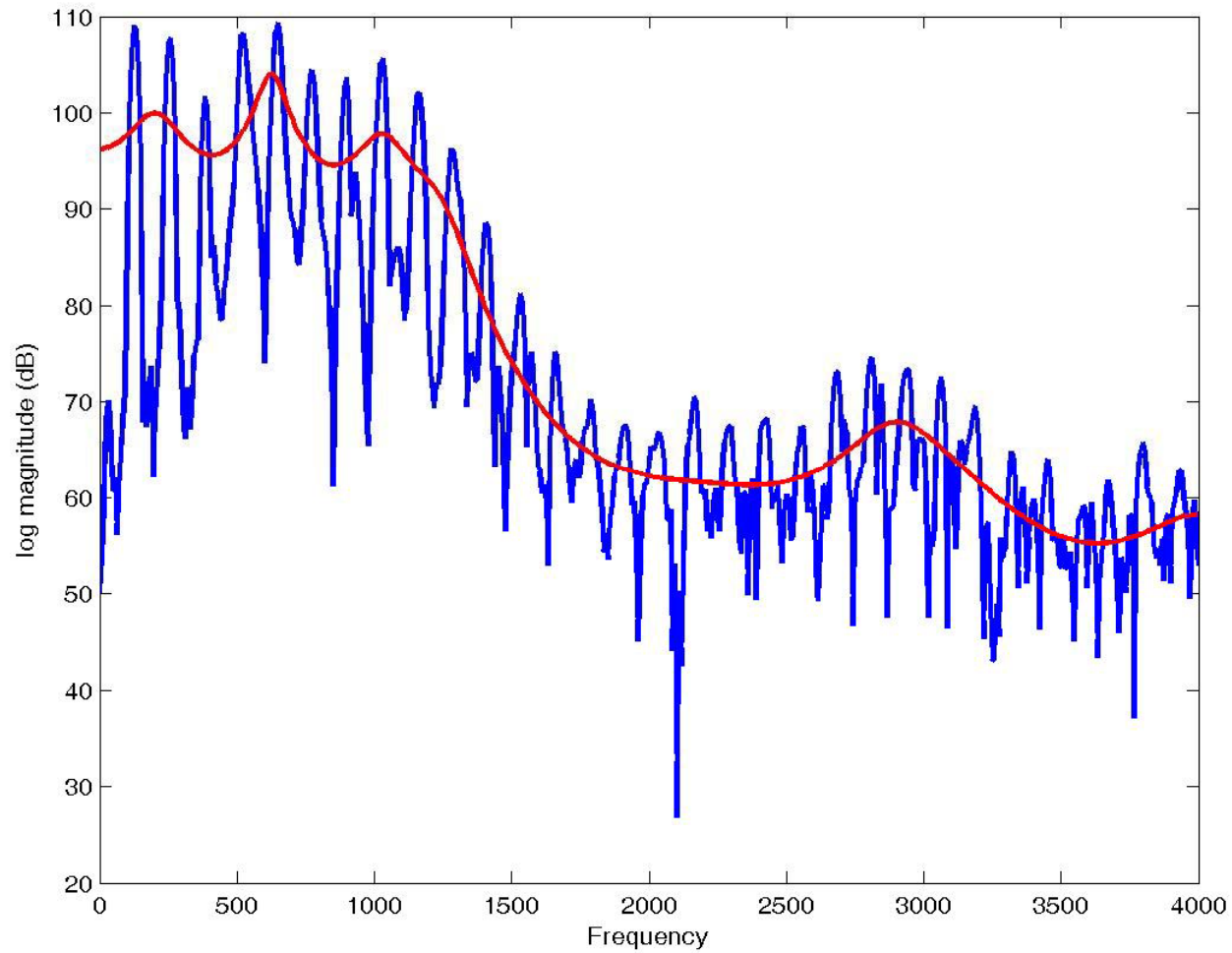
Frequency Response of Speech for LPC order p = 16
