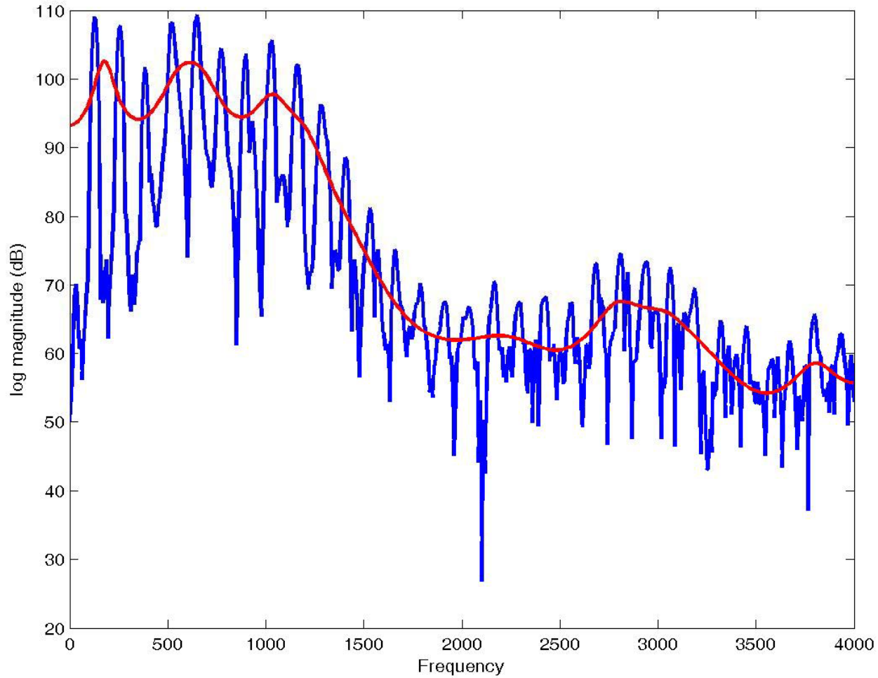
Frequency Response of Speech for LPC order p = 25
