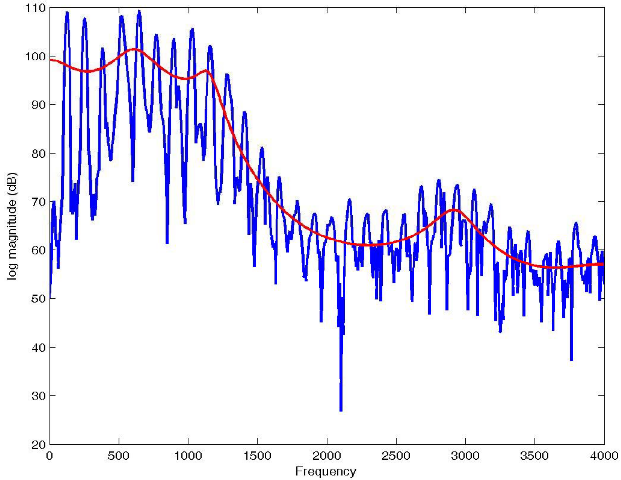
Frequency Response of Speech for LPC order p = 12
