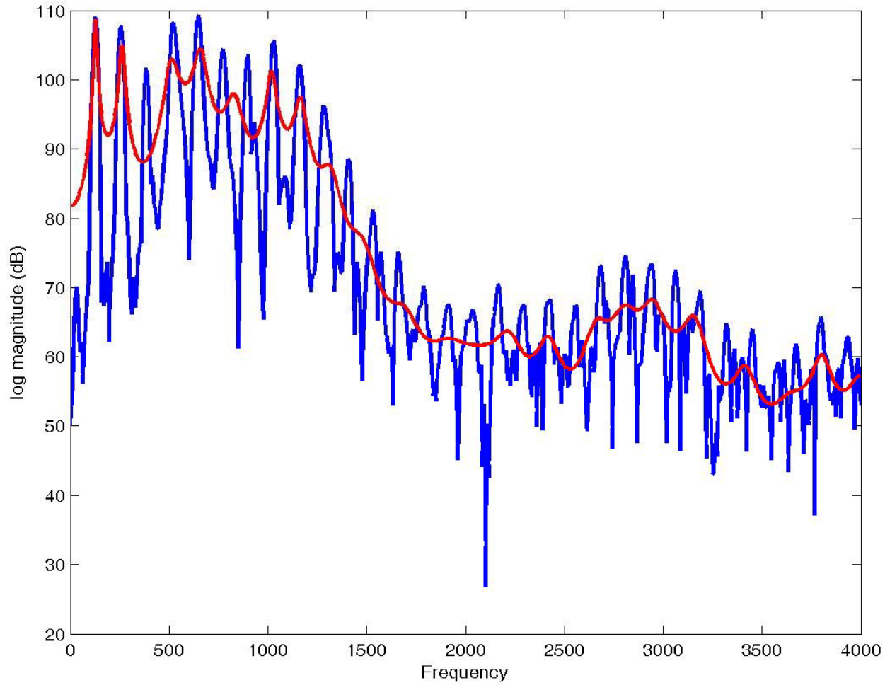
Frequency Response of Speech for LPC order p = 50
