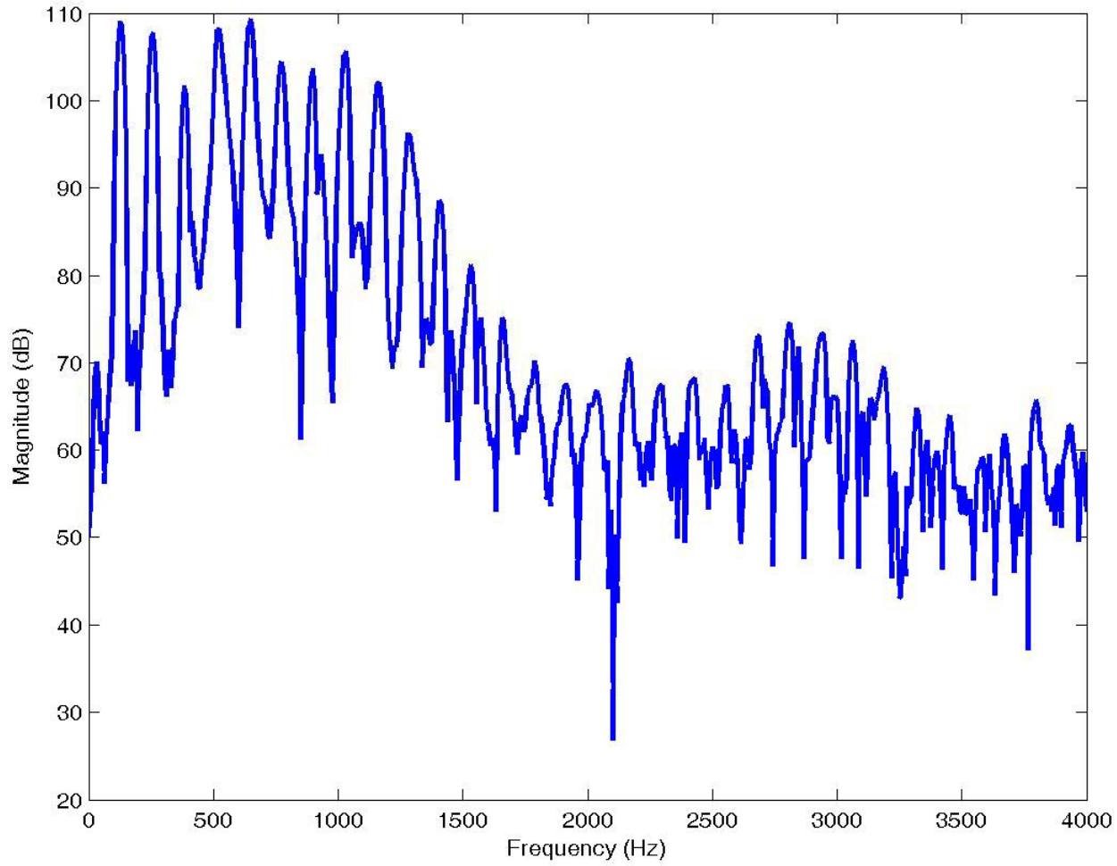
Frequency Spectrum of Speech Signal
