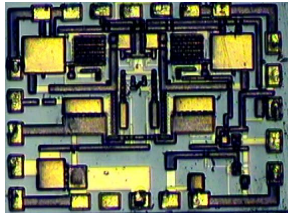
Fig.7 Chip Micrograph
