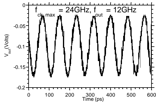
Fig. 14: Output waveform of the sum logic circuit for a 24 GHz clock input.
