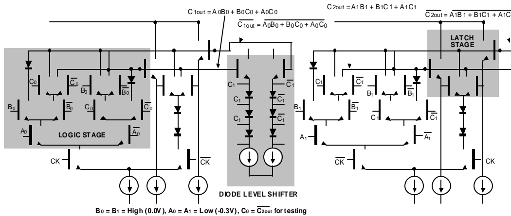
Fig. 11: 2-bit adder carry logic circuit.
