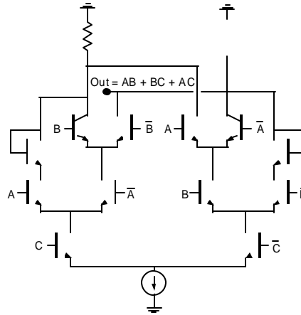
Fig. 5: Circuit diagram of the 3-level series-gated AND-OR gate that generates the carry output.
