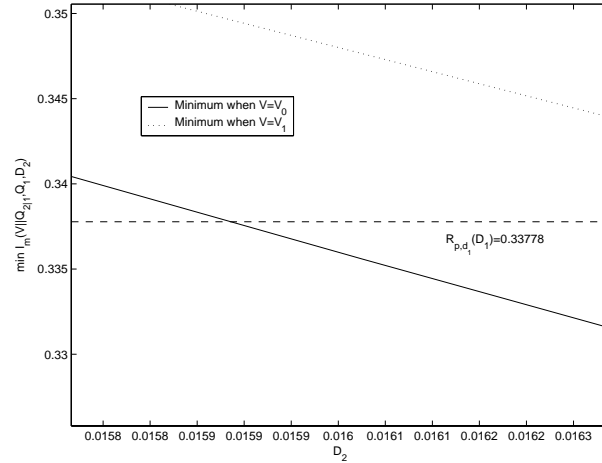
Fig. 3. Close-up of Figure 2 around D_2 = 0.016 .
