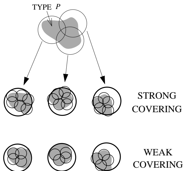
Fig. 1. Comparison of strong and weak hierarchical type covering schemes. Notice that the relaxed requirement of weak covering, i.e., that every vector \mathbf{x} must be jointly covered by a (D_1, D_2) -pair, may result in reduced number of D_2 -spheres compared to strong covering.
