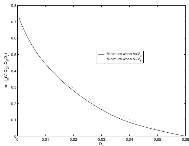
Fig. 2. Comparison of \min_{Q_{2|1} \in \mathcal{C}(\mathcal{Y}_2|\mathcal{Y}_1)} I_m(V_0||Q_{2|1}, Q_1, D_2) with \min_{Q_{2|1} \in \mathcal{C}(\mathcal{Y}_2|\mathcal{Y}_1)} I_m(V_1||Q_{2|1}, Q_1, D_2) . Clearly, the latter is strictly larger for a certain range of D_2 .
