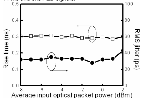
Figure 3: Rise time and RMS jitter of the PED rising edge, versus average input optical packet power (measured after the 90/10 coupler).
