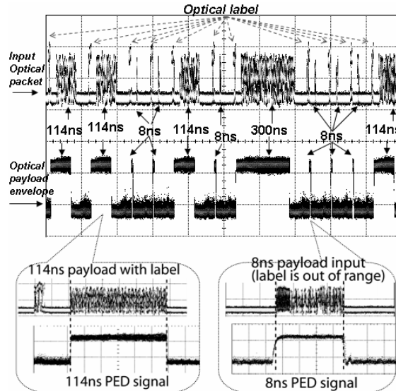
Figure 2: Input optical packets with labels and 8ns, 114ns, and 300ns long payloads (upper) and the corresponding PED signals (lower). Inset: zoom-in for 114ns and 8ns PED signals.
