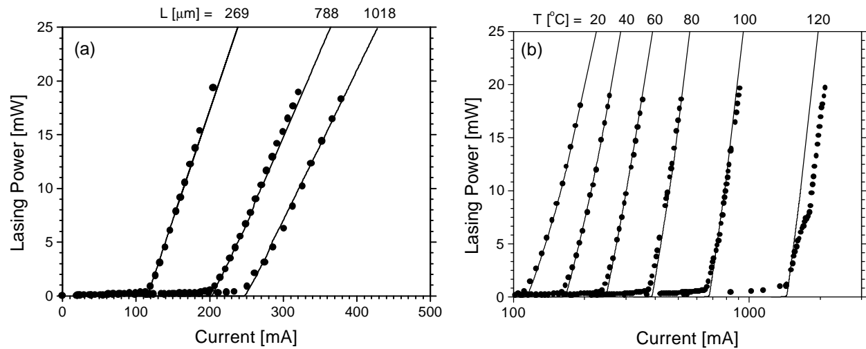
Fig. 2: Pulsed power vs. current characteristics (a) for various laser lengths L at T=20^\circ\text{C} and (b) for various stage temperatures T with L=269\mu\text{m} . Dots give measurements and lines give simulation results.
