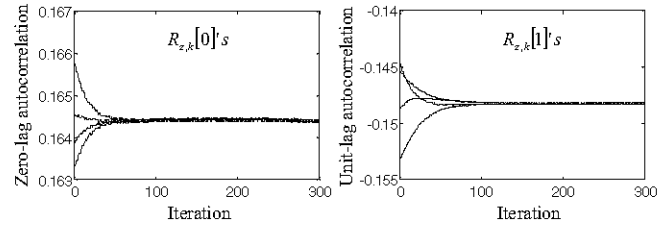
Figure 5. Equalization plot of measured R_{z,k}[0] 's (left) and R_{z,k}[1] 's (right) with a sinusoid input at 171.567MHz. Equalization is achieved after \sim 150 iterations.
