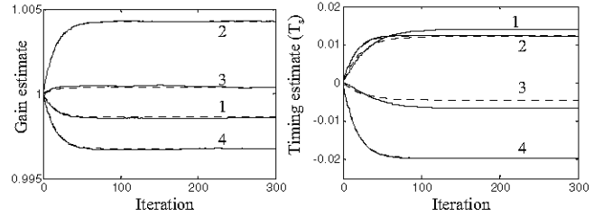
Figure 4. Convergence plot of gain (left) and timing (right) estimate with channel numbers shown. Solid lines represent measurement. Dotted lines denote predicted curves by (19) and (20) using intrinsic gain errors [0.9986 1.0043 1.0004 0.9968] and timing errors [0.0120 T_s 0.0123 T_s -0.0046 T_s -0.0198 T_s ] at 171.567MHz characterized by a training method [13].
