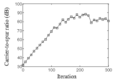
Figure 6. Measured carrier-to-spur ratio with a sine wave input at 171.567MHz. Only gain and timing mismatch spurs (marked as 'X' in Fig. 3) are considered. On achieving convergence, mismatch spurs are suppressed by \sim 50 dB down to \sim 80 dB below carrier.
