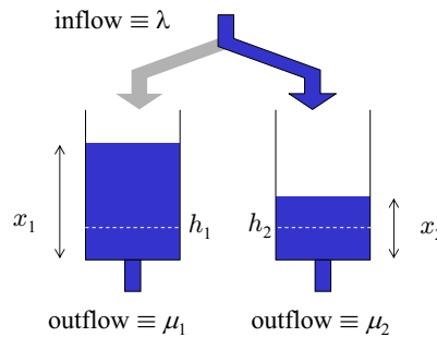
Figure 2. Two-tank system
