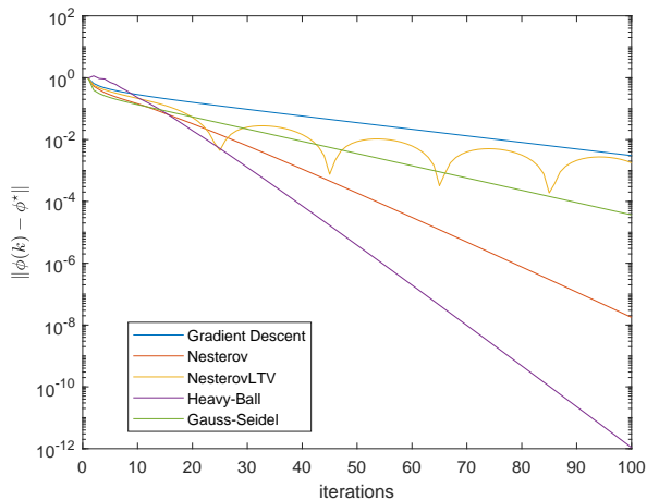
Fig. 6. Logarithmic evolution of the error norm for the PCO-based (Gradient Descent), Nesterov, LTV Nesterov, Heavy-Ball and Gauss-Seidel algorithms for a 20 node network.
