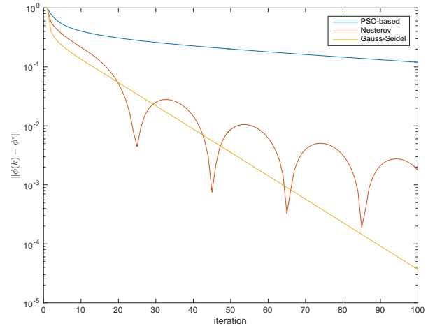
Fig. 4. Logarithmic evolution of the error norm for the PCO-based, Nesterov and Gauss-Seidel algorithms for the 20 node network.
