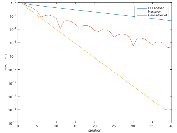
Fig. 3. Logarithmic evolution of the error norm for the PCO-based, Nesterov and Gauss-Seidel algorithms.
