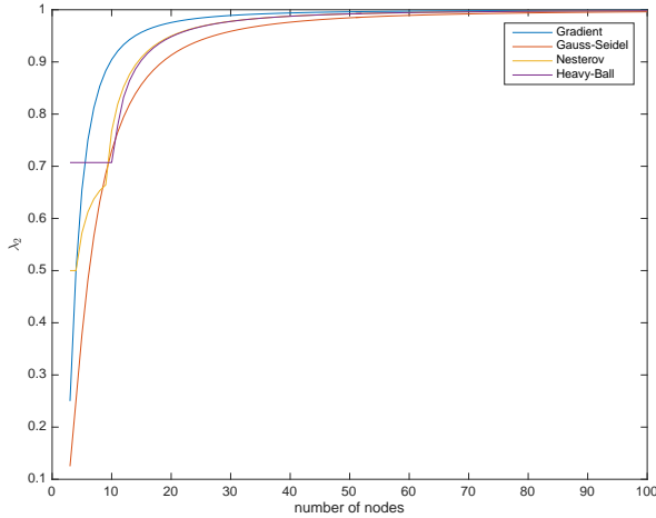
Fig. 2. The convergence rate \lambda_2 for the different algorithms depending on the number of nodes n .
