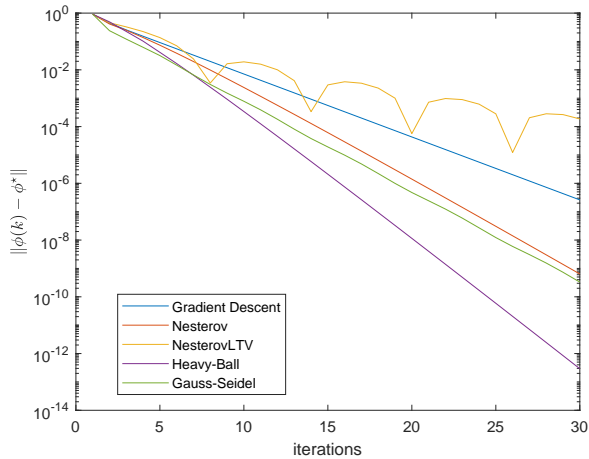
Fig. 5. Logarithmic evolution of the error norm for the PCO-based (Gradient Descent), Nesterov, LTV Nesterov, Heavy-Ball and Gauss-Seidel algorithms for a 6 node network.
