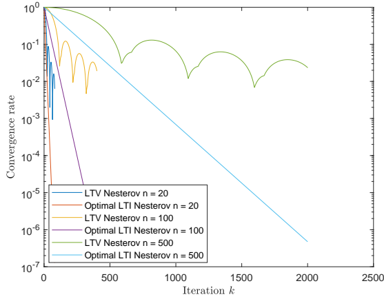
Fig. 1. Logarithmic evolution of the convergence rate for the time-varying Nesterov (LTVnesterov) and optimal fixed parameter Nesterov for networks sizes of 20, 100 and 500.
