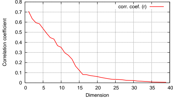
Fig. 1. Sorted correlation coefficient plot for audio and lip texture CCA analysis.
