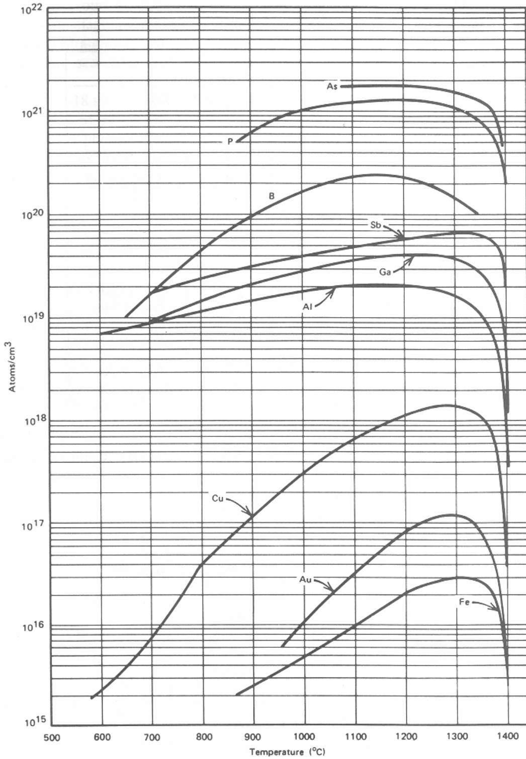
Fig. 2.20 The solid solubility of impurities in silicon.
