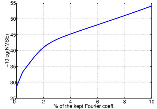
Fig. 4. Characterizing the sparsity of the channel of Fig. 3.
