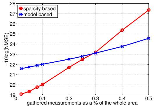
Fig. 8. Performance of the model-based and sparsity-based approaches for a 2D channel in the basement of the ECE building.
