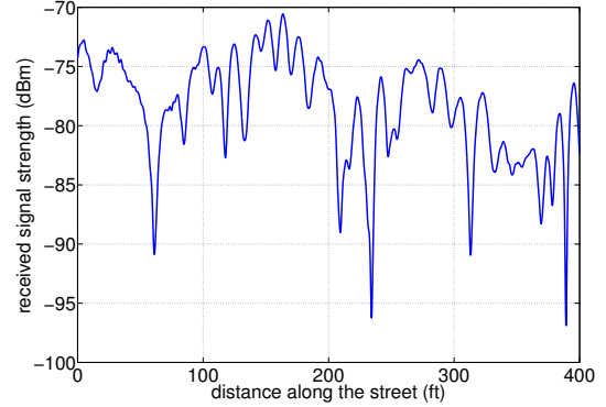
Fig. 3. channel measurement across a street in San Francisco [14].
